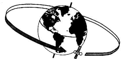
Fig 4-5 An Equatorial Orbit
